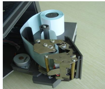
(4) Insert the release paper to the rewriter
