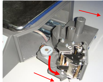
(2) Take out the printer, and open the turnable printing assembly
