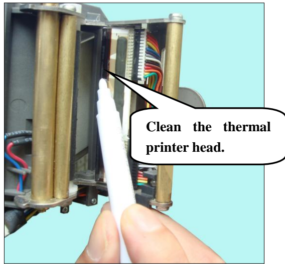
② Clean the thermal printer head.
